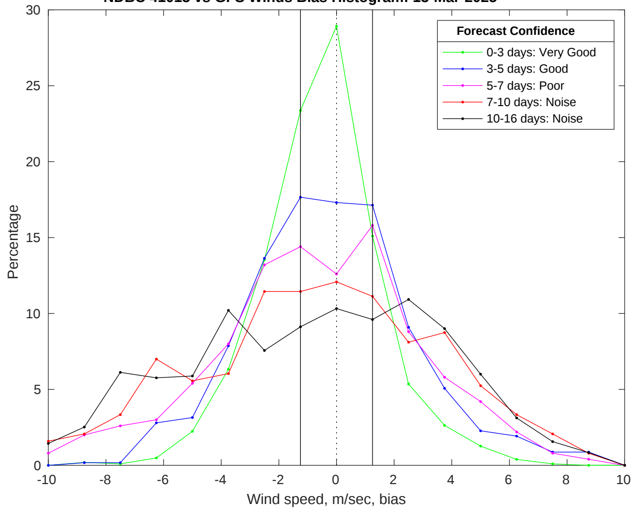
NDBC 41013 vs GFS Winds Bias Histogram: 13-Mar-2025
