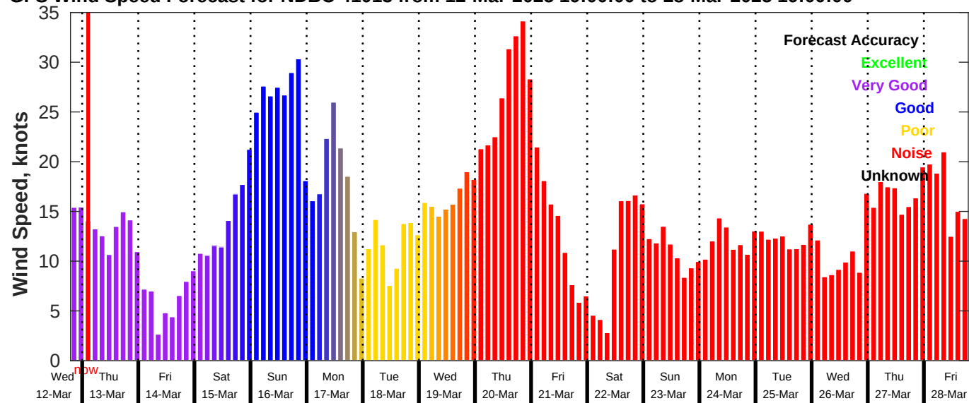
GFS Wind Speed Forecast for NDBC 41013 from 12-Mar-2025 19:00:00 to 28-Mar-2025 19:00:00
