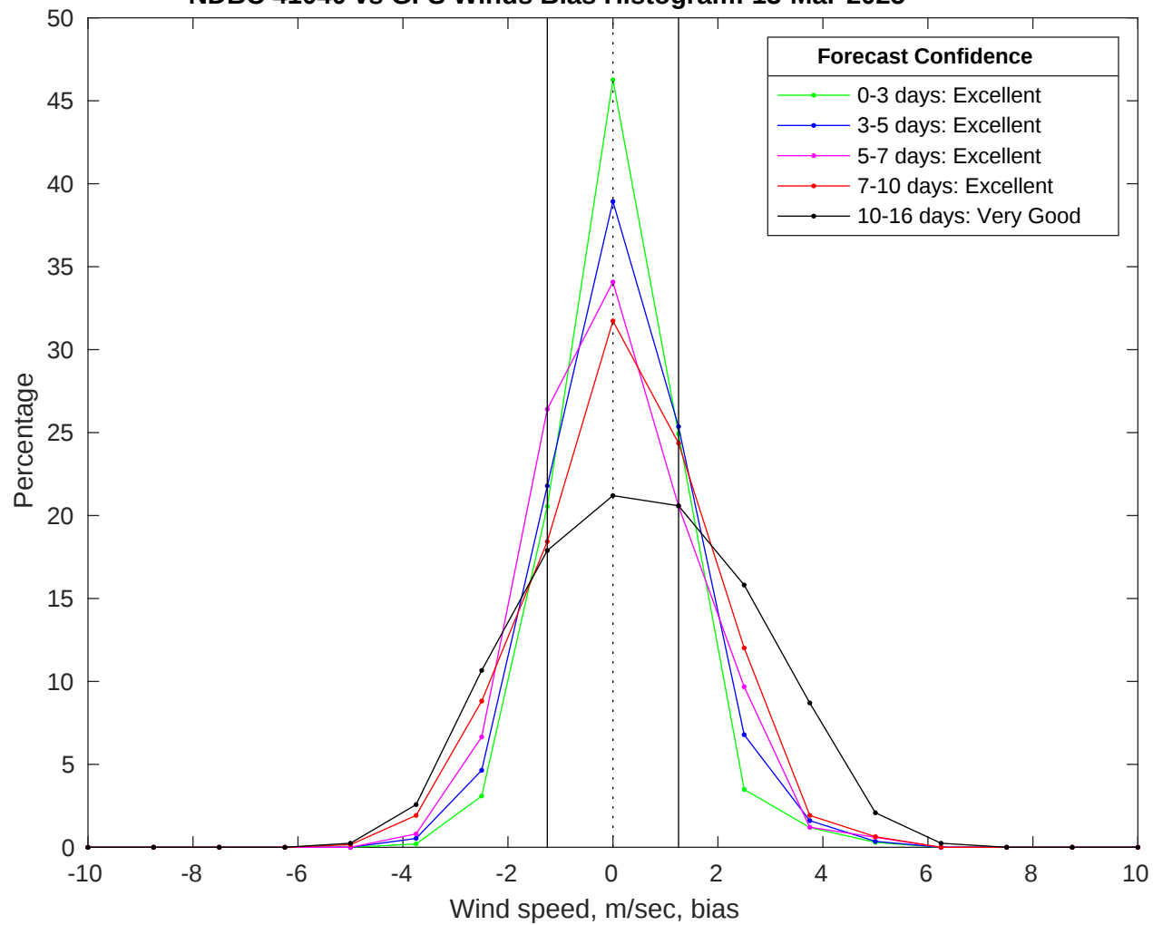
NDBC 41040 vs GFS Winds Bias Histogram: 13-Mar-2025
