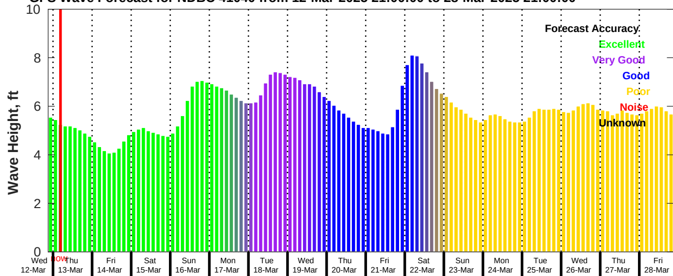
GFS Wave Forecast for NDBC 41040 from 12-Mar-2025 21:00:00 to 28-Mar-2025 21:00:00
