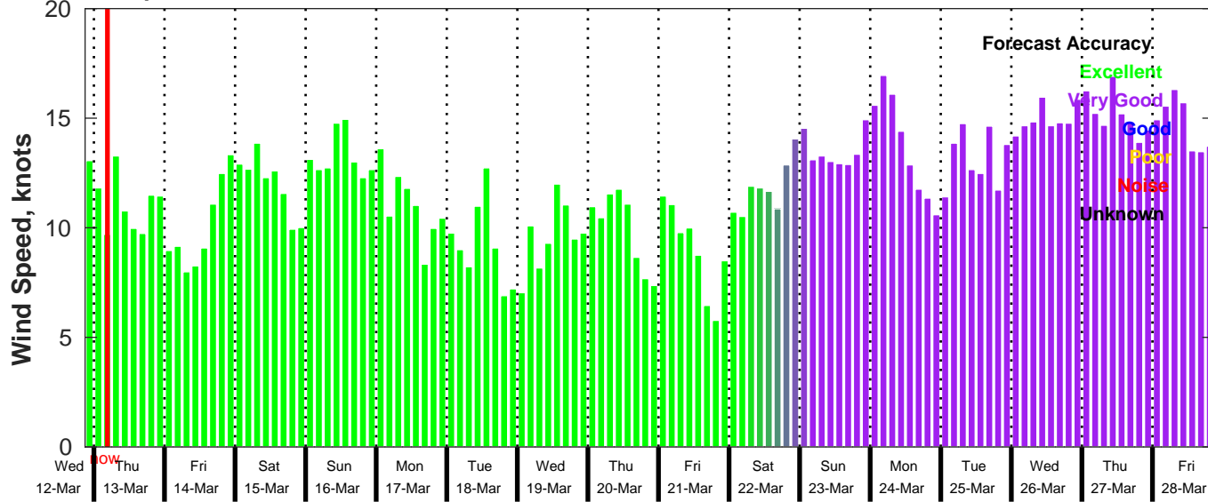
GFS Wind Speed Forecast for NDBC 41040 from 12-Mar-2025 21:00:00 to 28-Mar-2025 21:00:00
