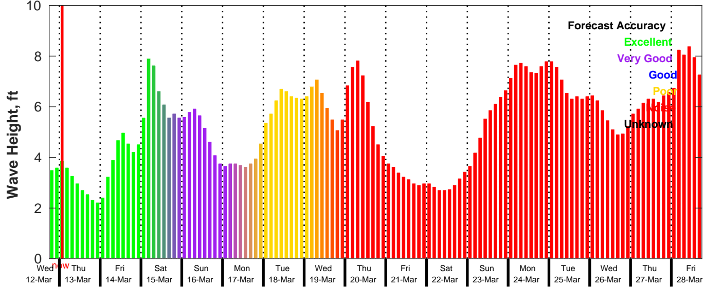
GFS Wave Forecast for NDBC 42019 from 12-Mar-2025 18:00:00 to 28-Mar-2025 18:00:00
