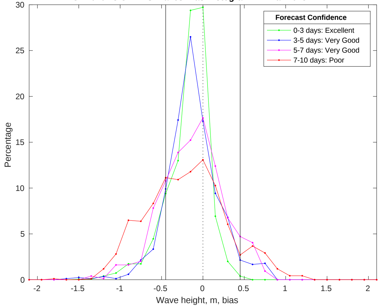
NDBC 42020 vs CMEMS Waves Bias Histogram: 12-Mar-2025
