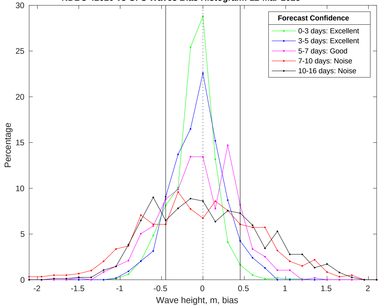
NDBC 42020 vs GFS Waves Bias Histogram: 12-Mar-2025
