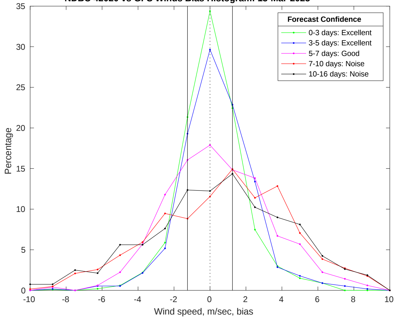
NDBC 42020 vs GFS Winds Bias Histogram: 13-Mar-2025
