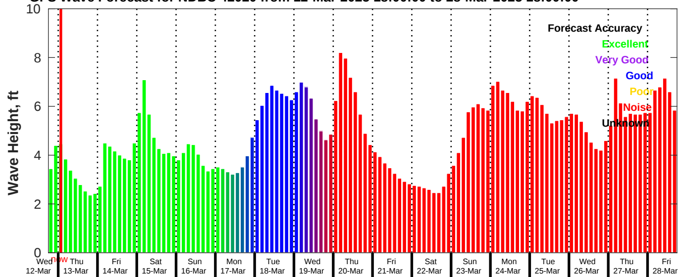
GFS Wave Forecast for NDBC 42020 from 12-Mar-2025 18:00:00 to 28-Mar-2025 18:00:00
