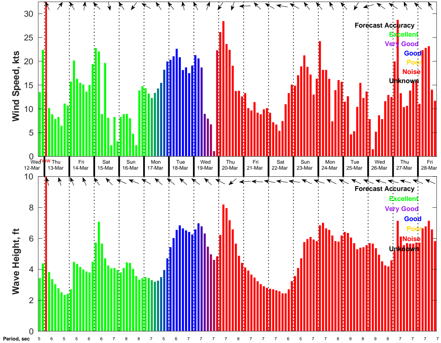
Wind & Wave Forecast for NDBC 42020 from 12-Mar-2025 18:00:00 to 28-Mar-2025 18:00:00
