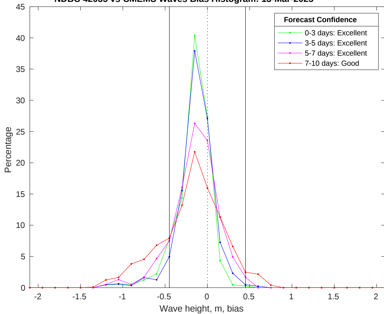
NDBC 42035 vs CMEMS Waves Bias Histogram: 13-Mar-2025
