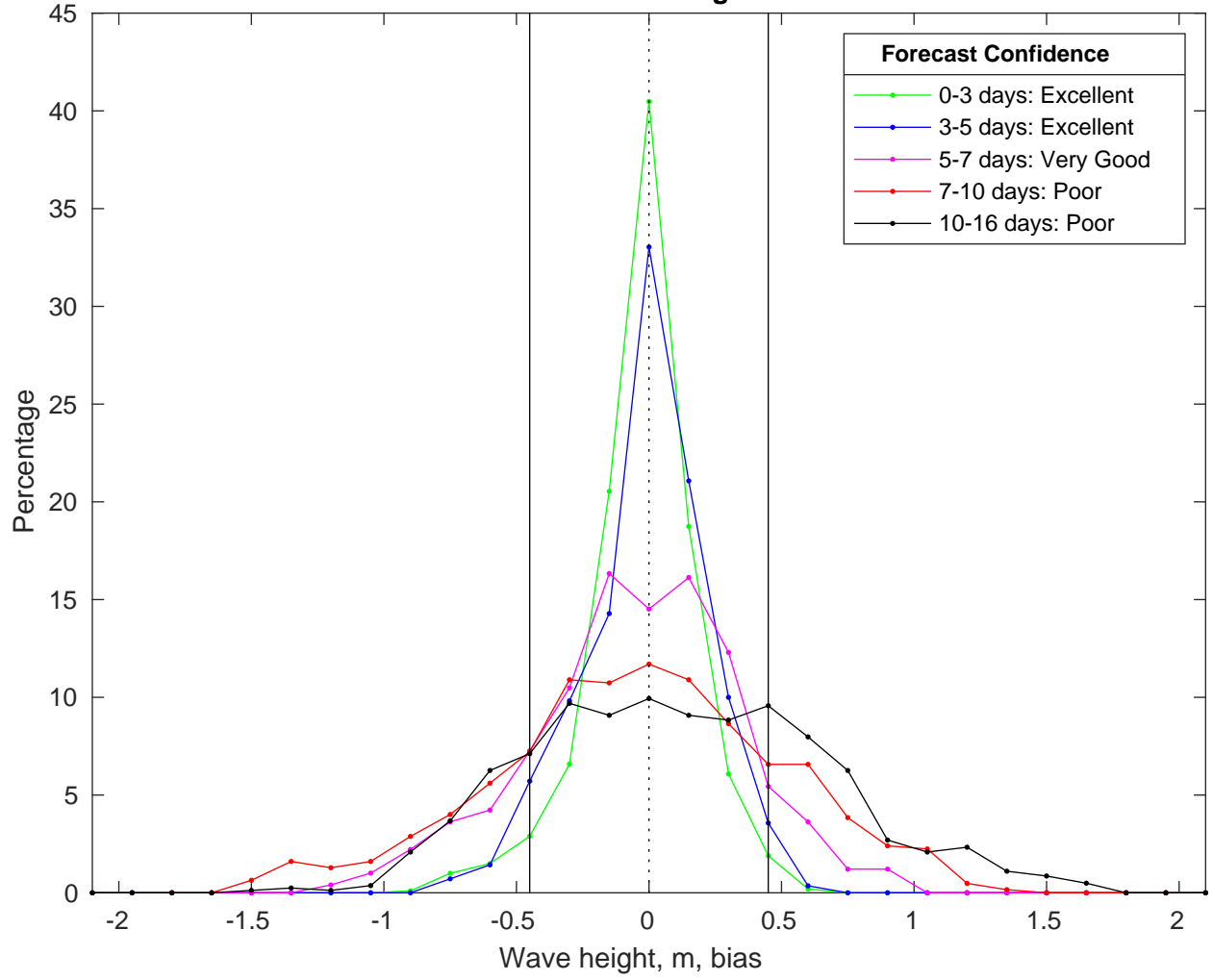
NDBC 42035 vs GFS Waves Bias Histogram: 13-Mar-2025
