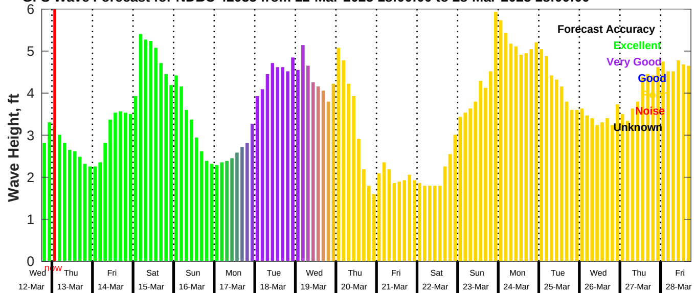
GFS Wave Forecast for NDBC 42035 from 12-Mar-2025 18:00:00 to 28-Mar-2025 18:00:00
