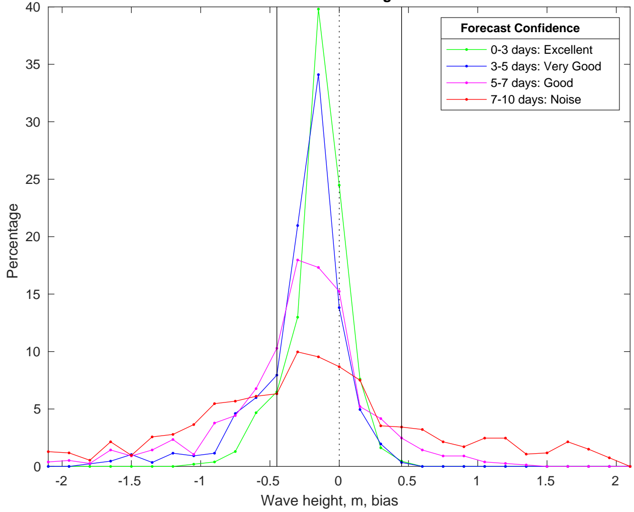
NDBC 42036 vs CMEMS Waves Bias Histogram: 13-Mar-2025
