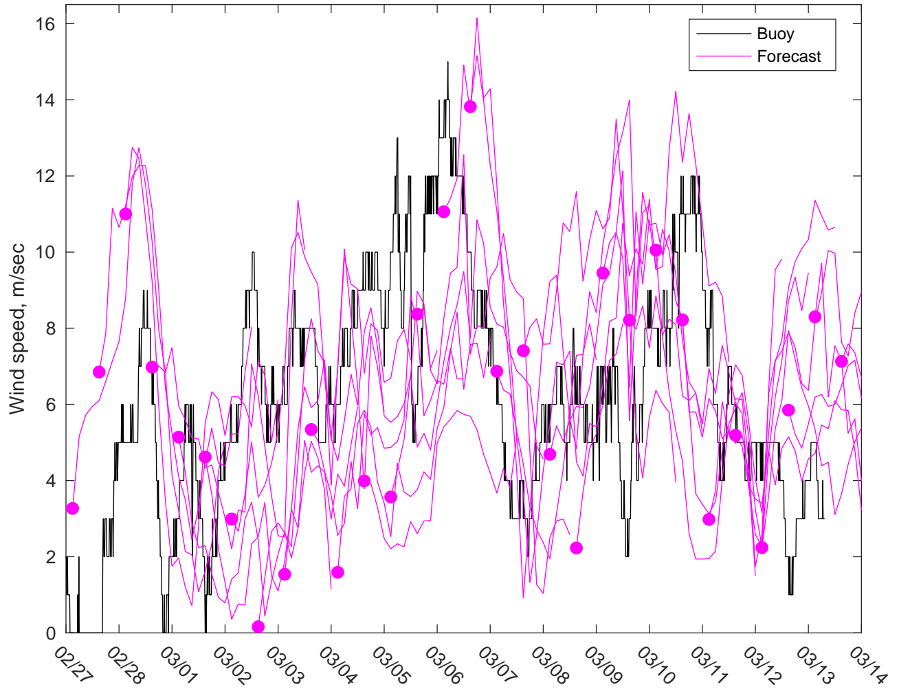
NDBC 42036 vs GFS Winds: 7 to 10 day forecast
