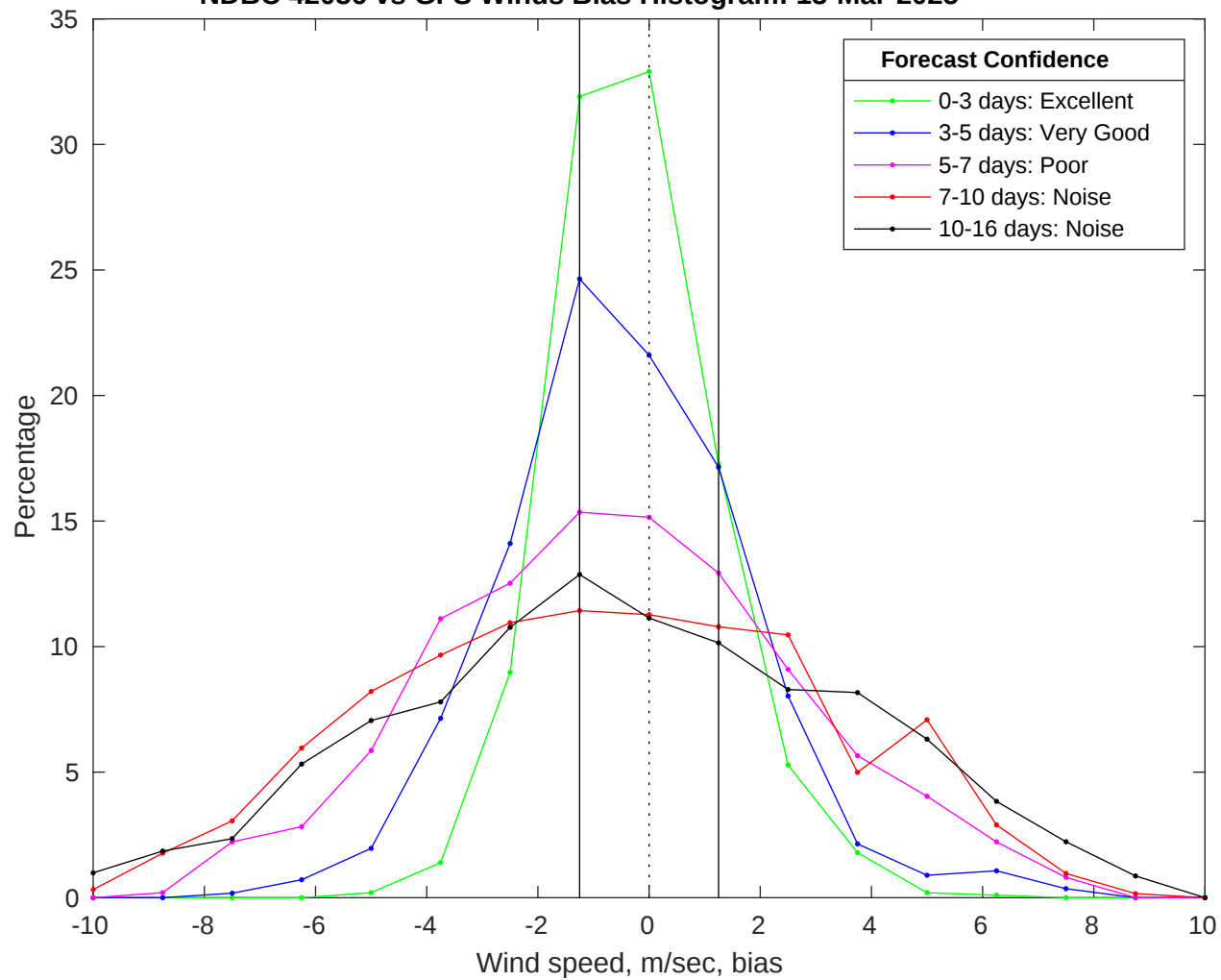
NDBC 42036 vs GFS Winds Bias Histogram: 13-Mar-2025
