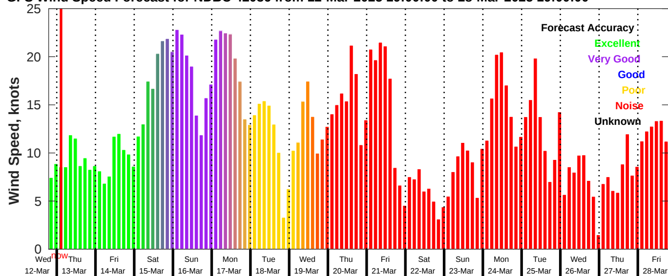
GFS Wind Speed Forecast for NDBC 42036 from 12-Mar-2025 19:00:00 to 28-Mar-2025 19:00:00
