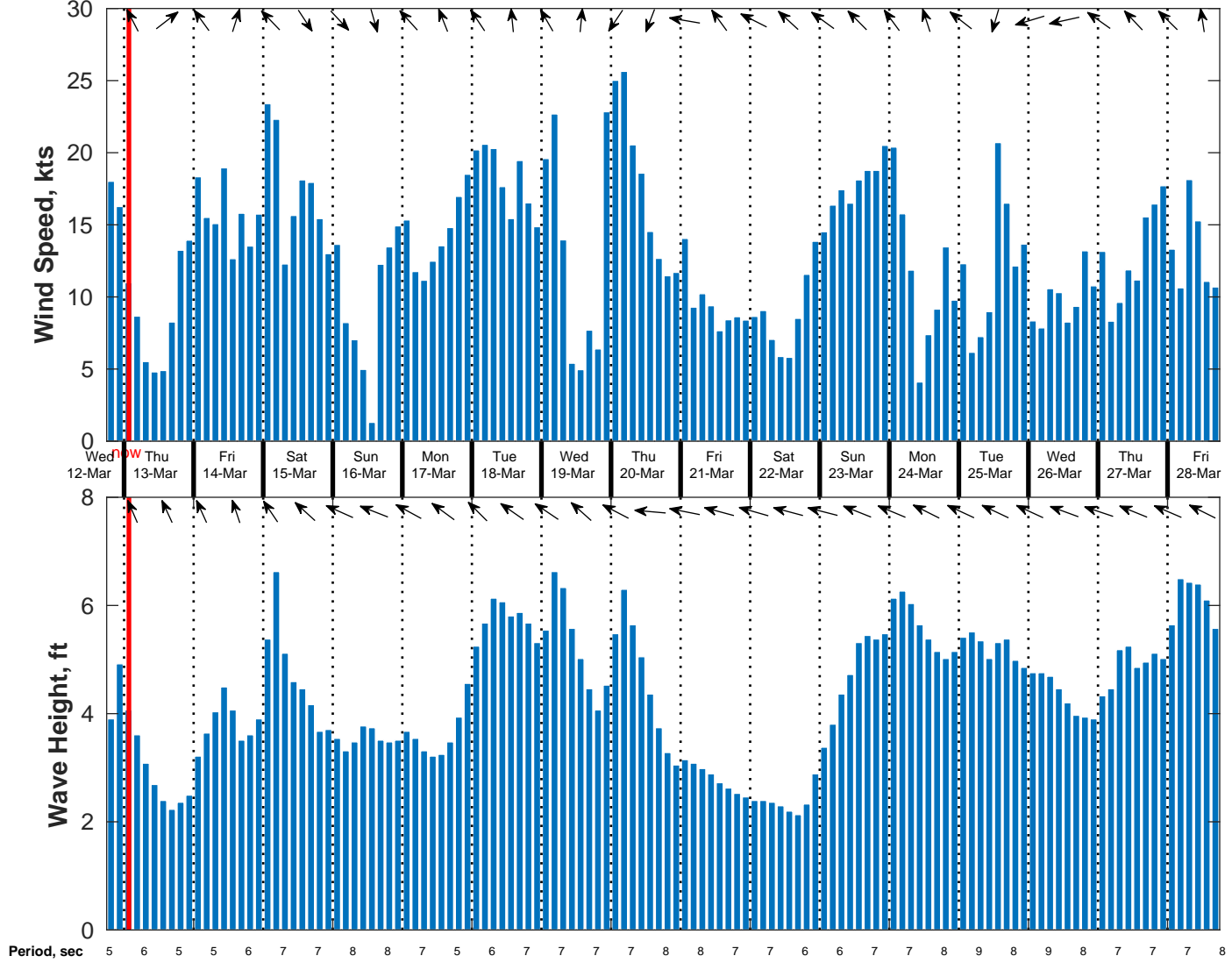
Wind & Wave Forecast for NDBC 42092 from 12-Mar-2025 18:00:00 to 28-Mar-2025 18:00:00
