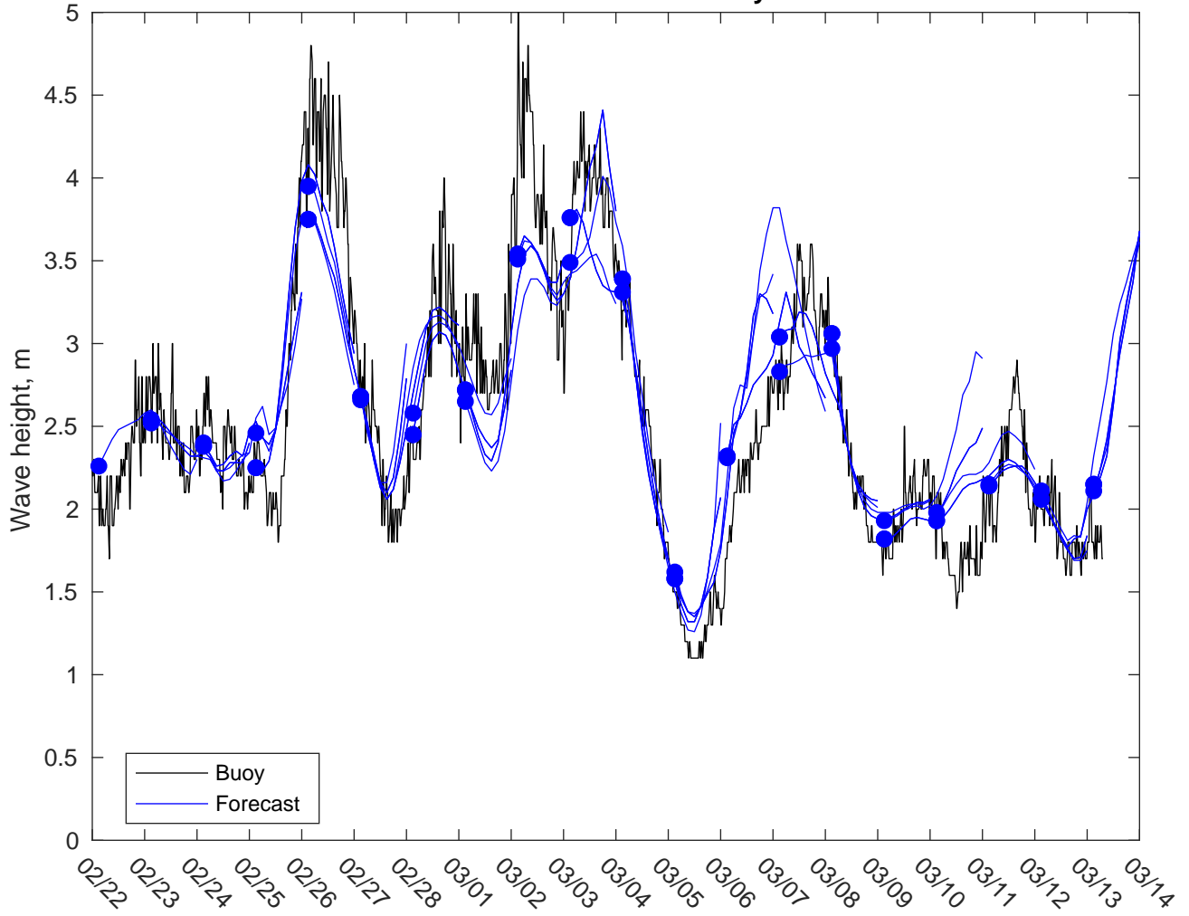
NDBC 46011 vs CMEMS Waves: 3 to 5 day forecast
