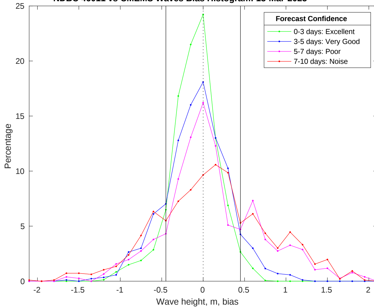
NDBC 46011 vs CMEMS Waves Bias Histogram: 13-Mar-2025
