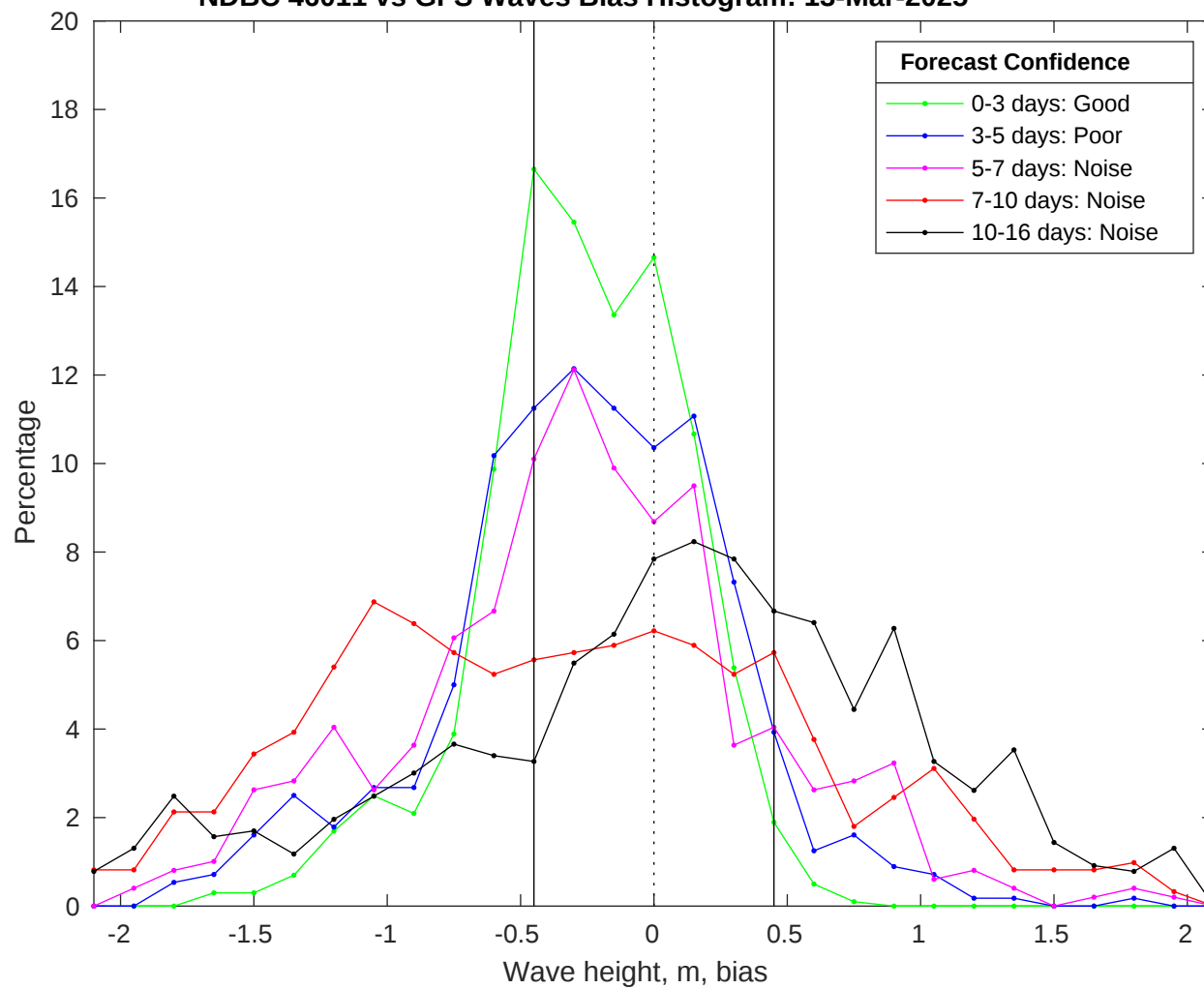
NDBC 46011 vs GFS Waves Bias Histogram: 13-Mar-2025
