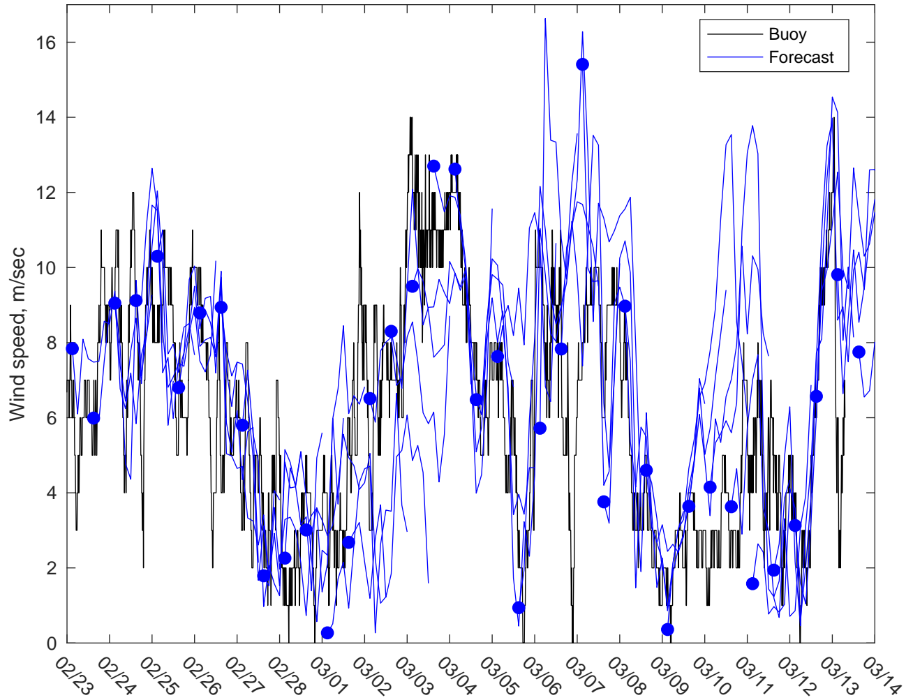
NDBC 46011 vs GFS Winds: 3 to 5 day forecast
