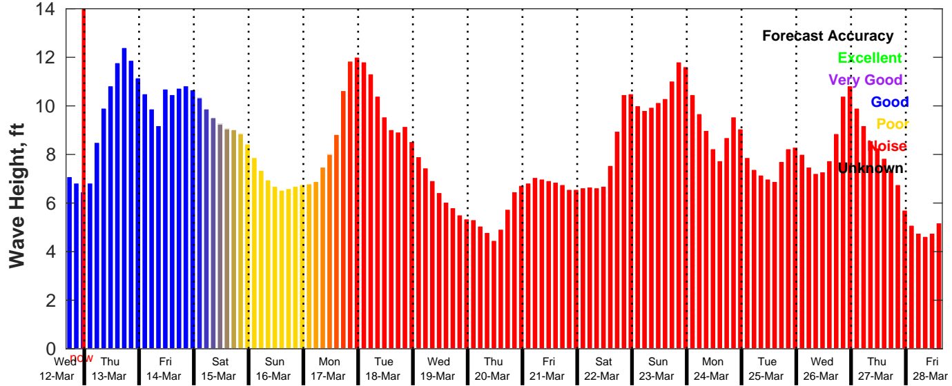
GFS Wave Forecast for NDBC 46011 from 12-Mar-2025 16:00:00 to 28-Mar-2025 16:00:00
