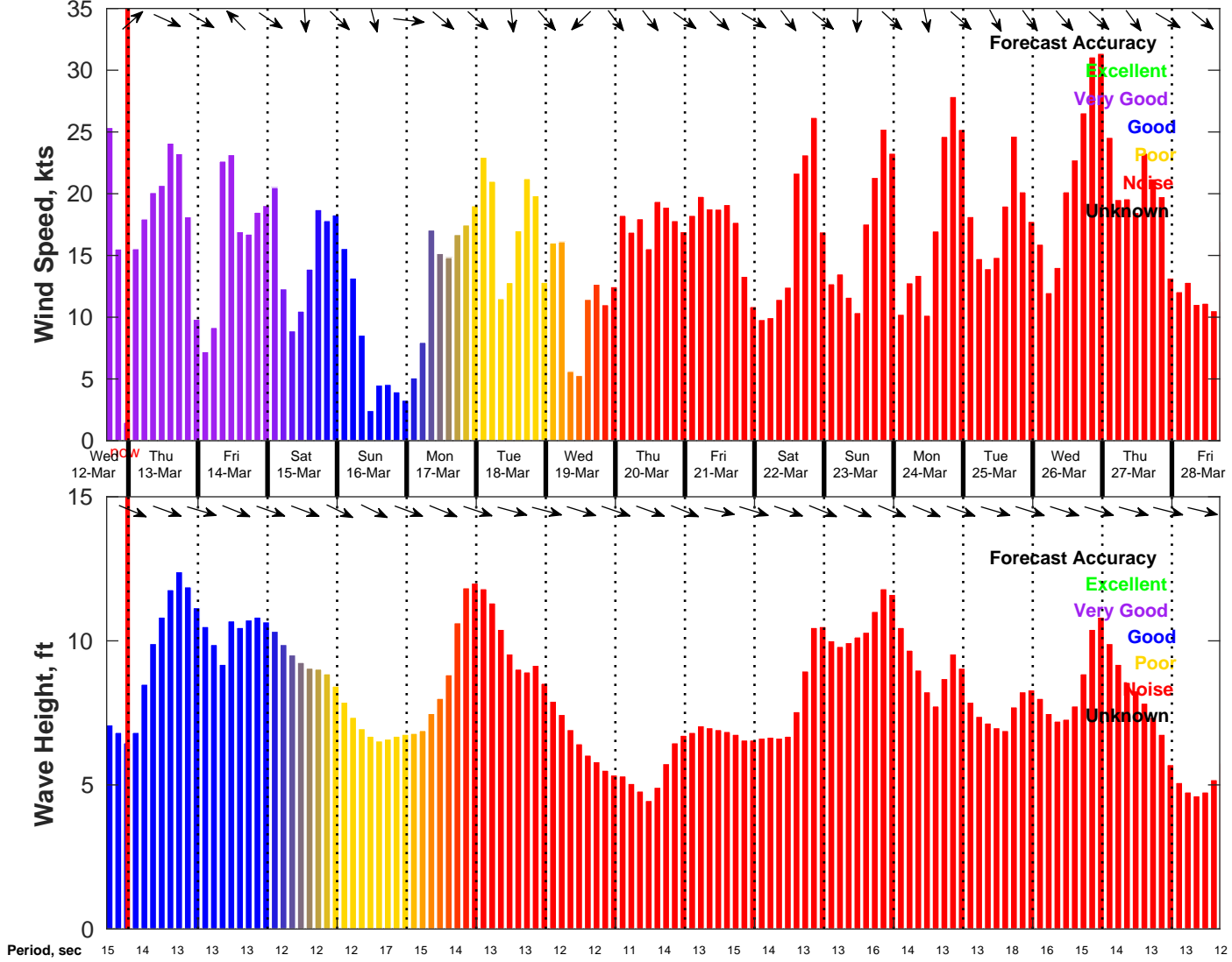
Wind & Wave Forecast for NDBC 46011 from 12-Mar-2025 16:00:00 to 28-Mar-2025 16:00:00
