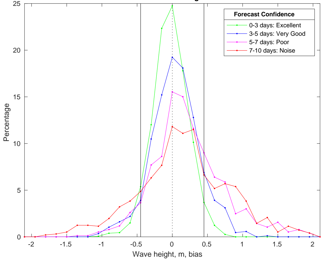
NDBC 46028 vs CMEMS Waves Bias Histogram: 13-Mar-2025
