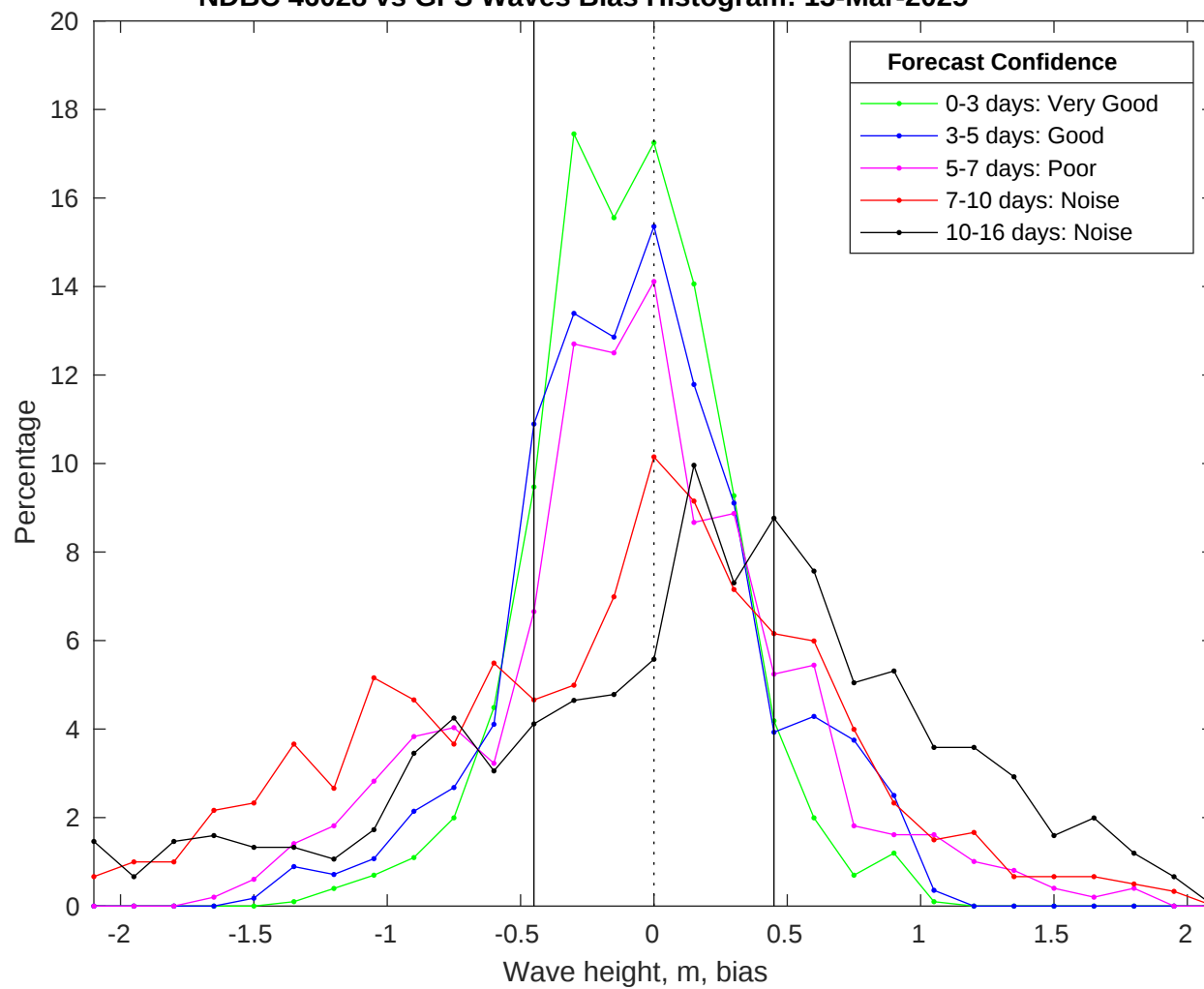
NDBC 46028 vs GFS Waves Bias Histogram: 13-Mar-2025
