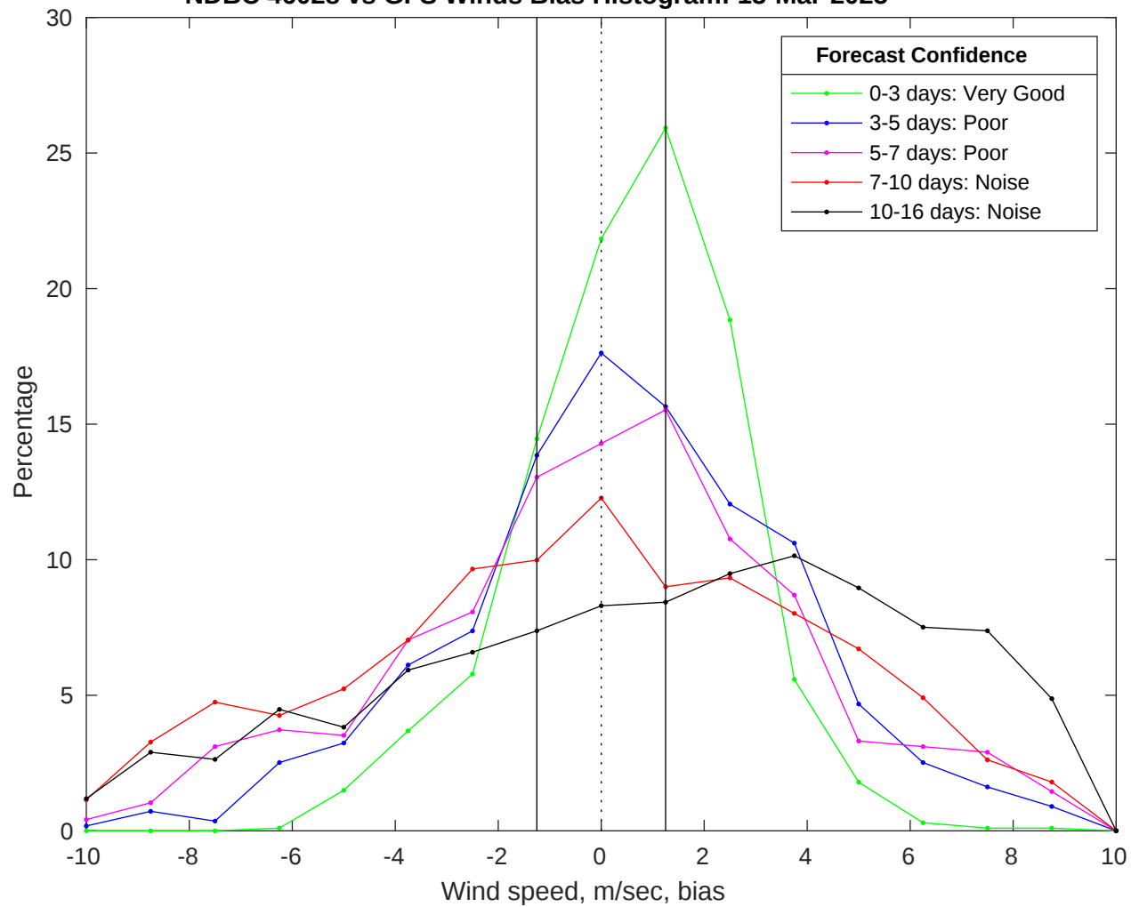
NDBC 46028 vs GFS Winds Bias Histogram: 13-Mar-2025
