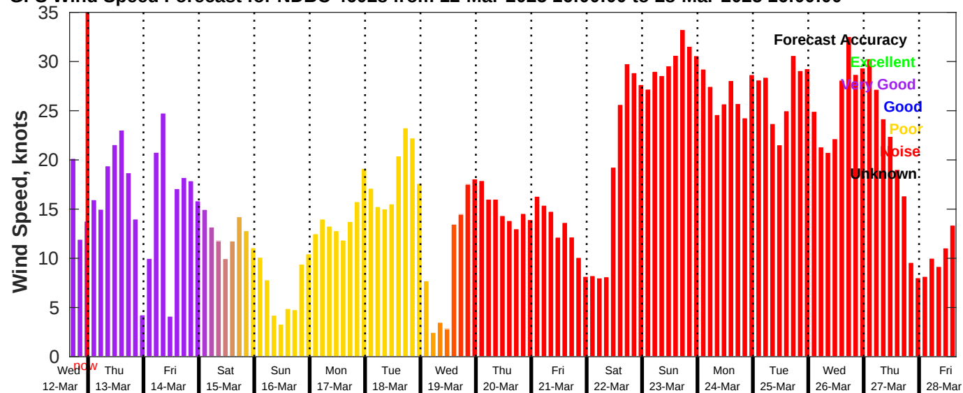
GFS Wind Speed Forecast for NDBC 46028 from 12-Mar-2025 16:00:00 to 28-Mar-2025 16:00:00
