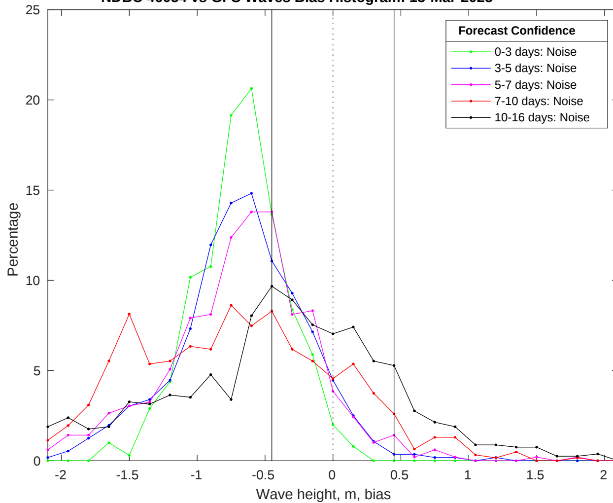
NDBC 46054 vs GFS Waves Bias Histogram: 13-Mar-2025
