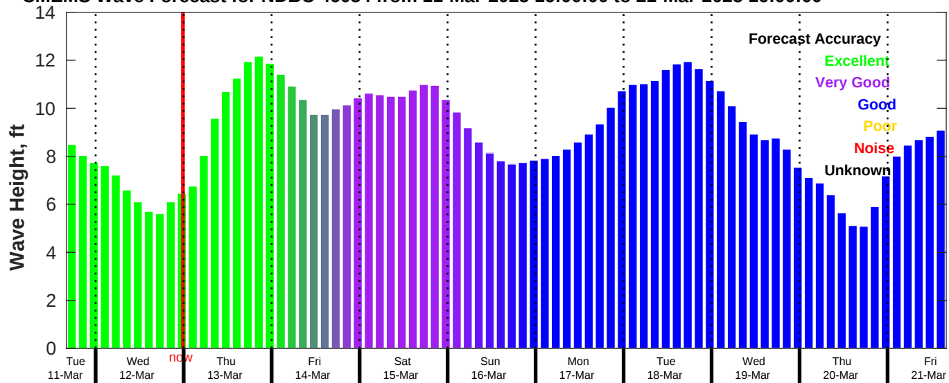
CMEMS Wave Forecast for NDBC 46054 from 11-Mar-2025 16:00:00 to 21-Mar-2025 16:00:00
