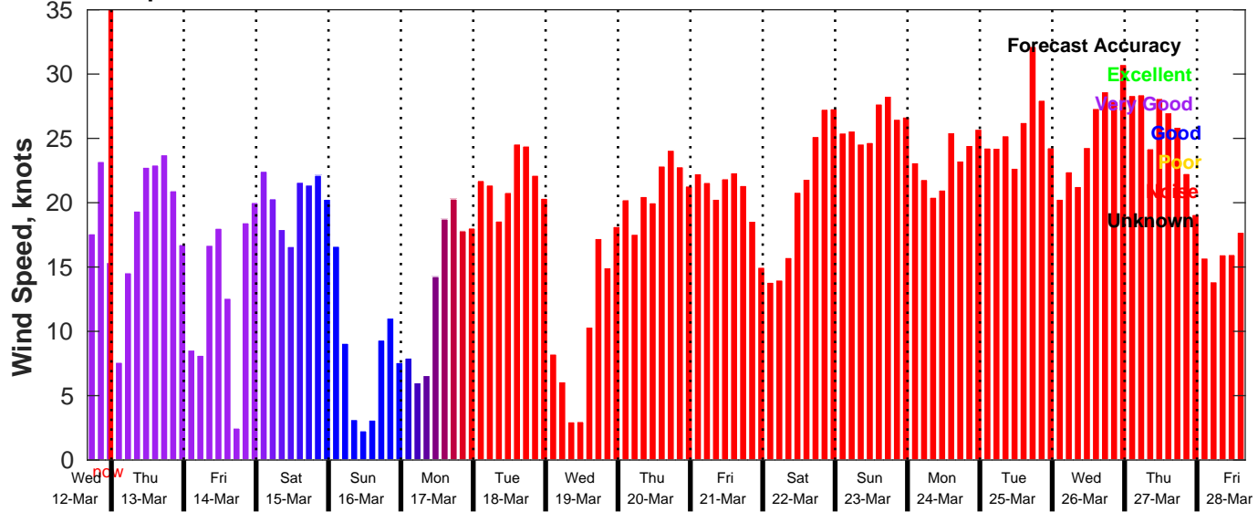
GFS Wind Speed Forecast for NDBC 46054 from 12-Mar-2025 16:00:00 to 28-Mar-2025 16:00:00
