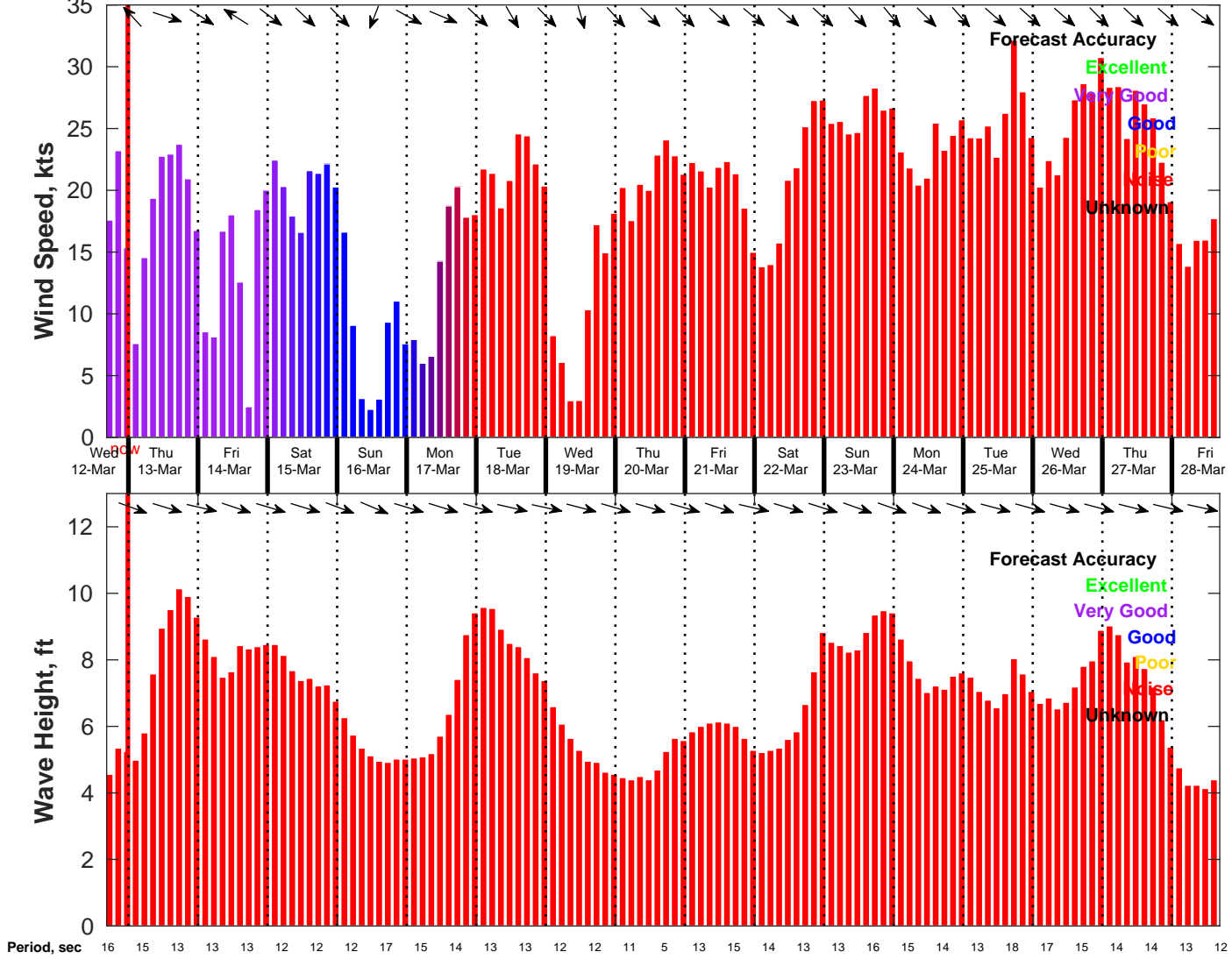
Wind & Wave Forecast for NDBC 46054 from 12-Mar-2025 16:00:00 to 28-Mar-2025 16:00:00
