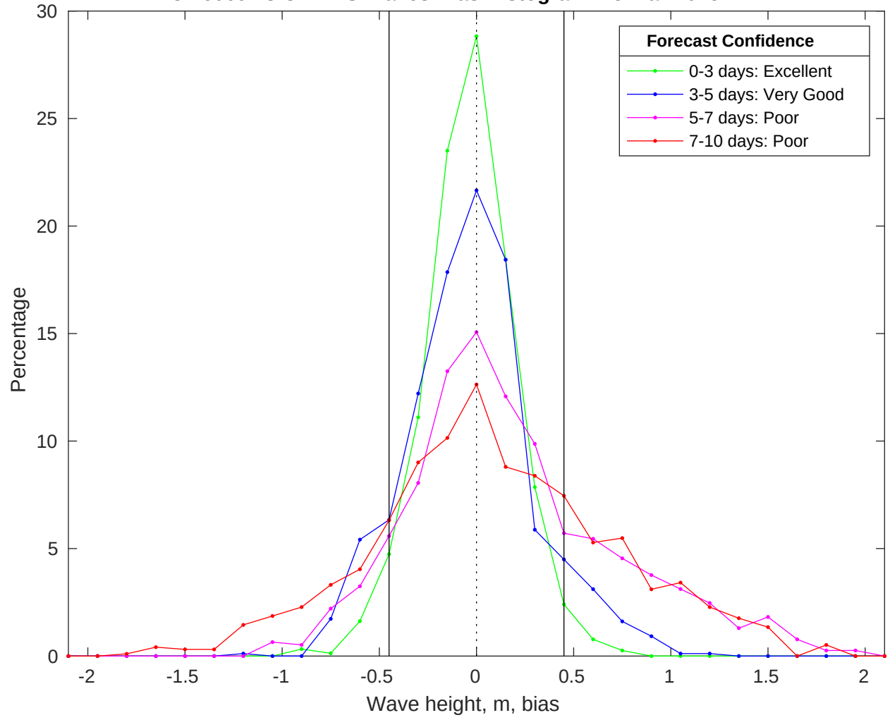
NDBC 46069 vs CMEMS Waves Bias Histogram: 13-Mar-2025
