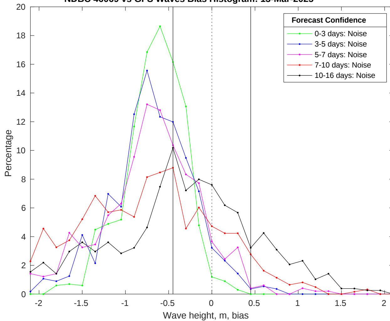
NDBC 46069 vs GFS Waves Bias Histogram: 13-Mar-2025
