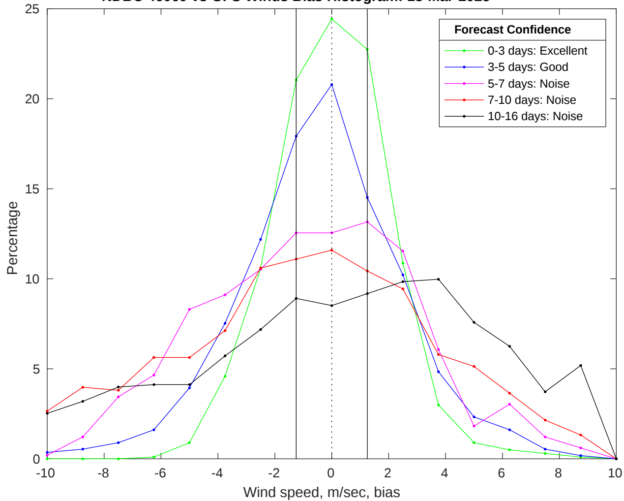
NDBC 46069 vs GFS Winds Bias Histogram: 13-Mar-2025
