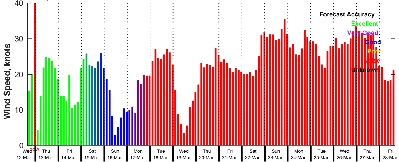
GFS Wind Speed Forecast for NDBC 46069 from 12-Mar-2025 16:00:00 to 28-Mar-2025 16:00:00
