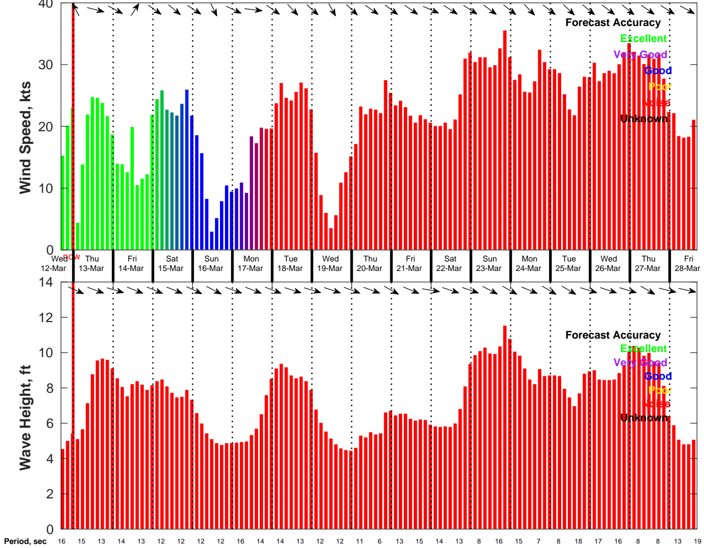
Wind & Wave Forecast for NDBC 46069 from 12-Mar-2025 16:00:00 to 28-Mar-2025 16:00:00
