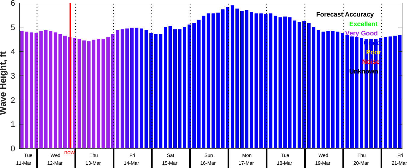
CMEMS Wave Forecast for NDBC 51209 from 11-Mar-2025 13:00:00 to 21-Mar-2025 13:00:00
