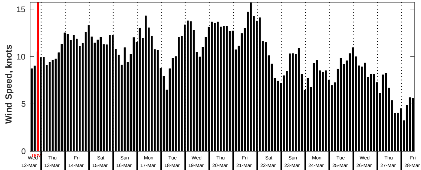
GFS Wind Speed Forecast for NDBC 51209 from 12-Mar-2025 13:00:00 to 28-Mar-2025 13:00:00
