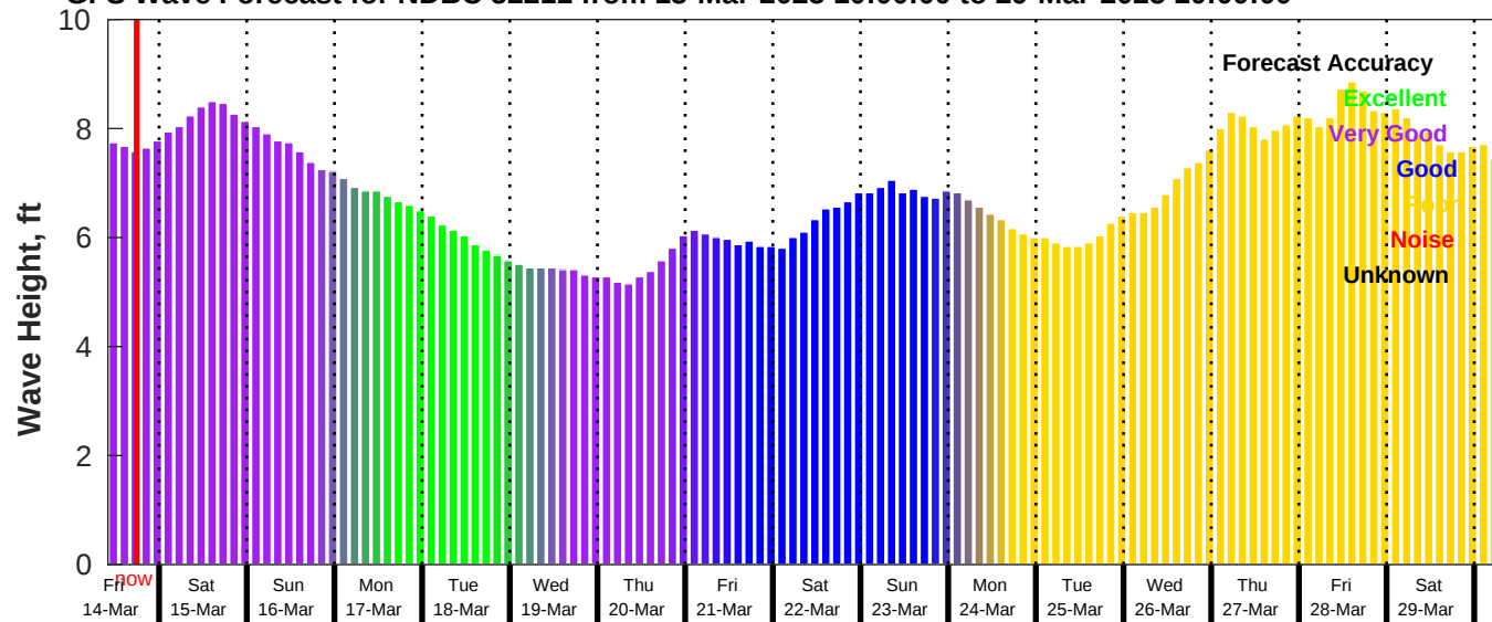
GFS Wave Forecast for NDBC 52211 from 13-Mar-2025 10:00:00 to 29-Mar-2025 10:00:00
