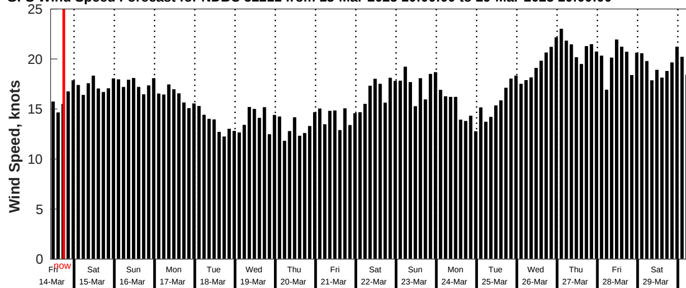
GFS Wind Speed Forecast for NDBC 52211 from 13-Mar-2025 10:00:00 to 29-Mar-2025 10:00:00
