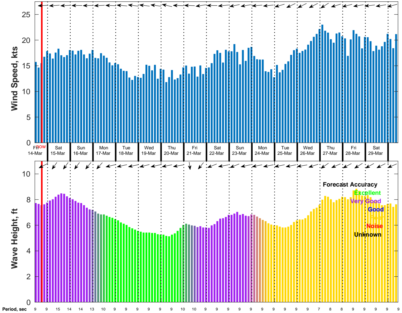
Wind & Wave Forecast for NDBC 52211 from 13-Mar-2025 10:00:00 to 29-Mar-2025 10:00:00
