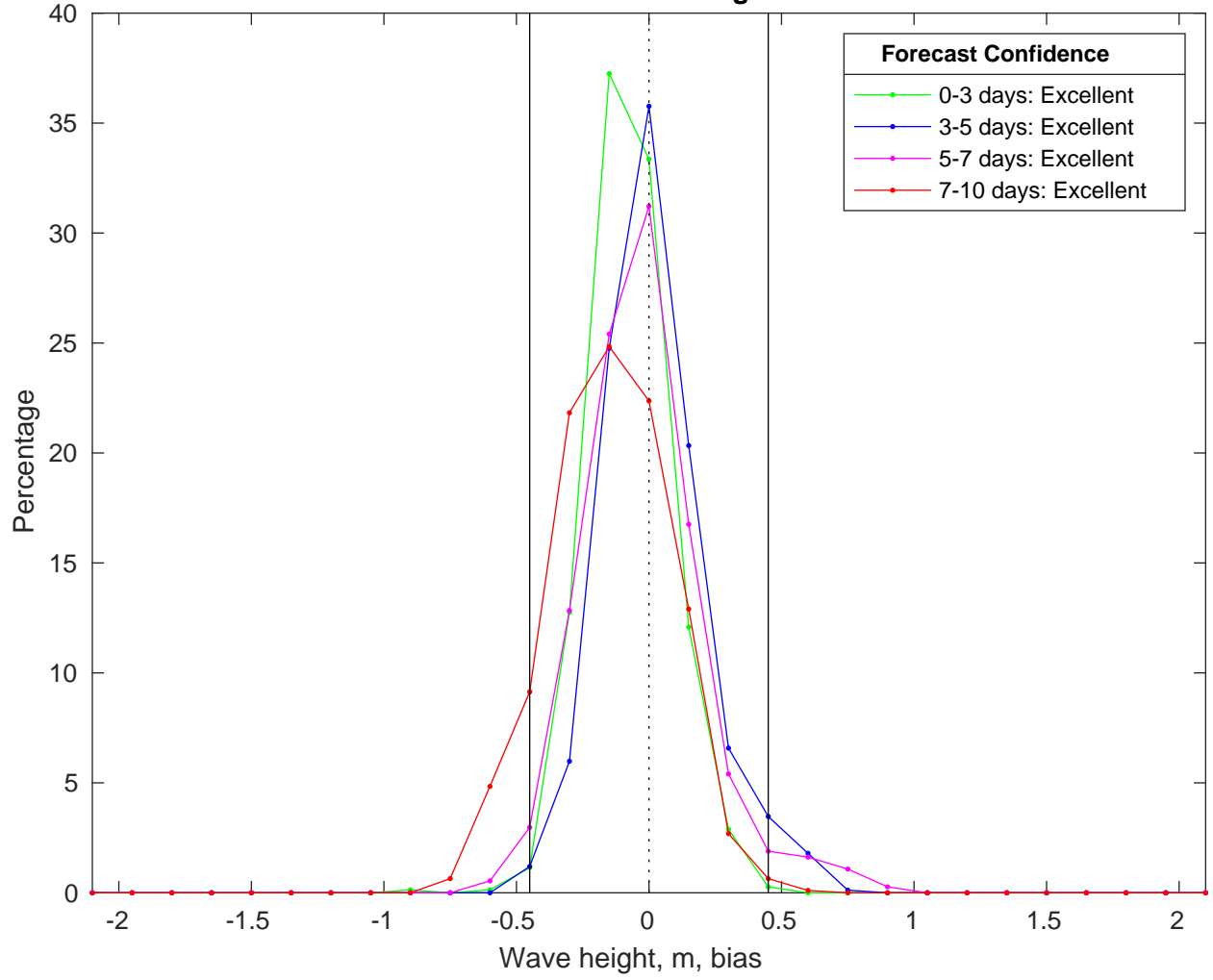
NDBC 52212 vs CMEMS Waves Bias Histogram: 13-Mar-2025
