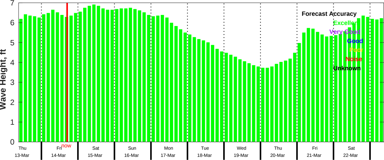
CMEMS Wave Forecast for NDBC 52212 from 12-Mar-2025 09:00:00 to 22-Mar-2025 09:00:00
