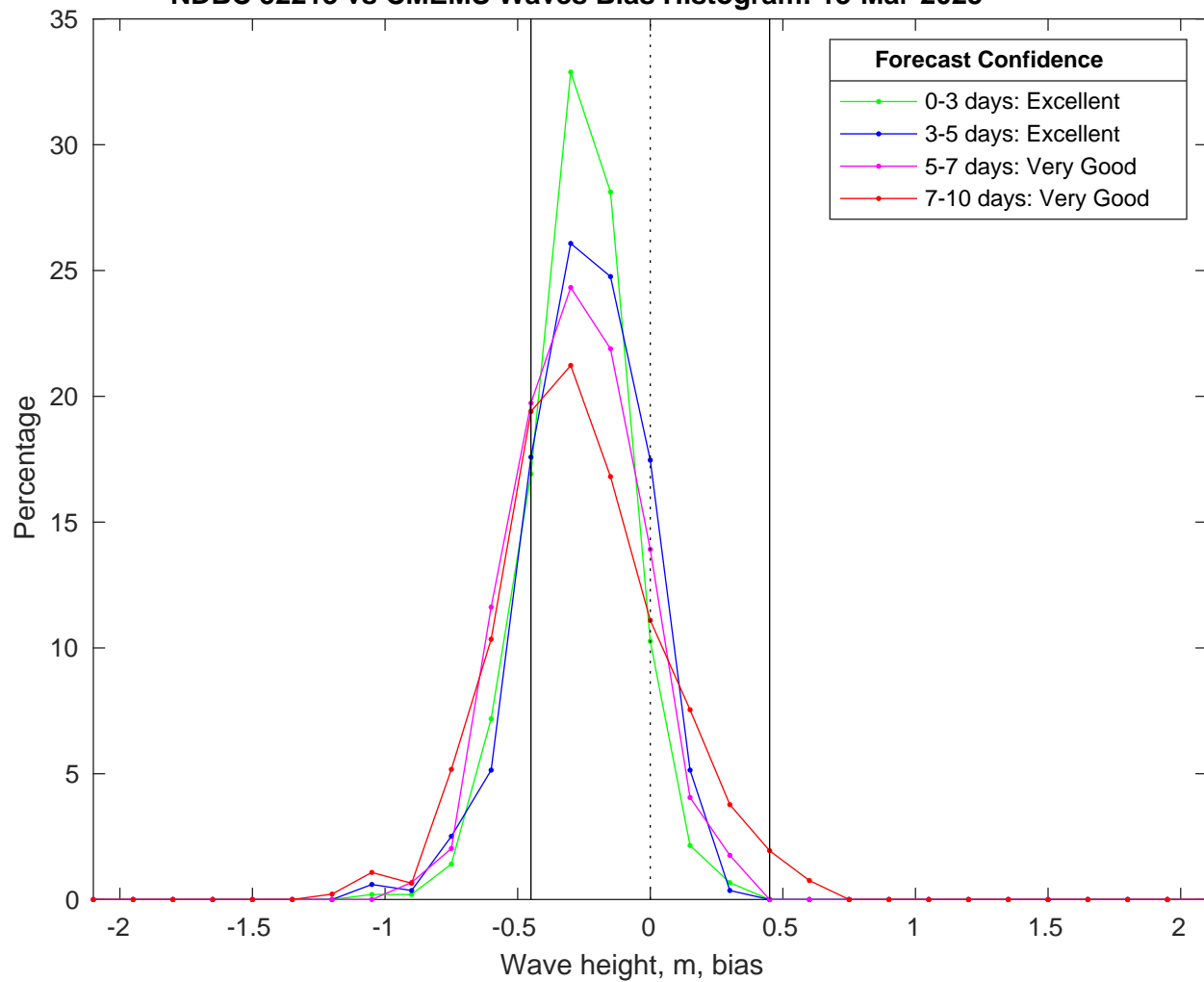
NDBC 52213 vs CMEMS Waves Bias Histogram: 13-Mar-2025
