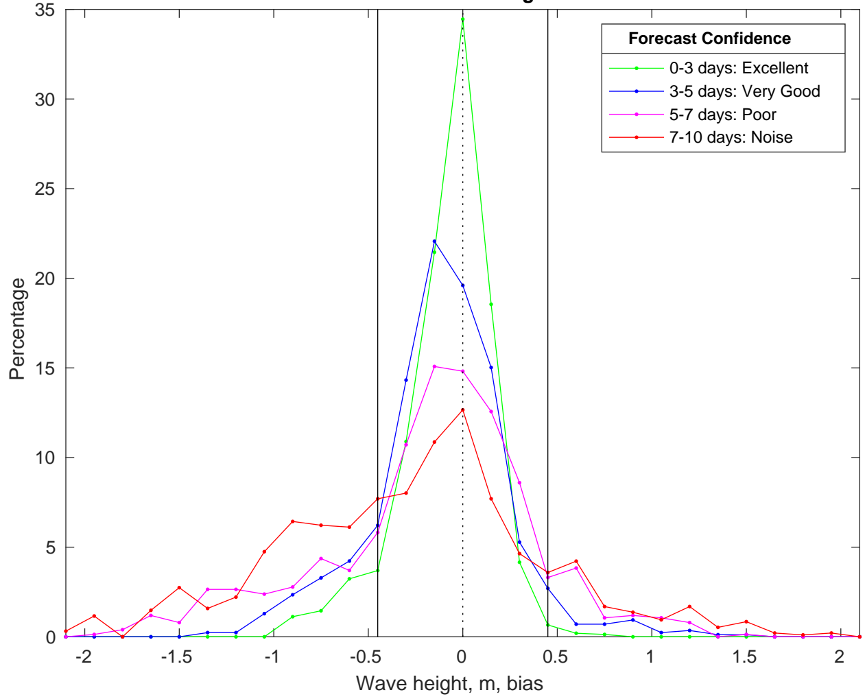
NDBC 41004 vs CMEMS Waves Bias Histogram: 14-Mar-2025
