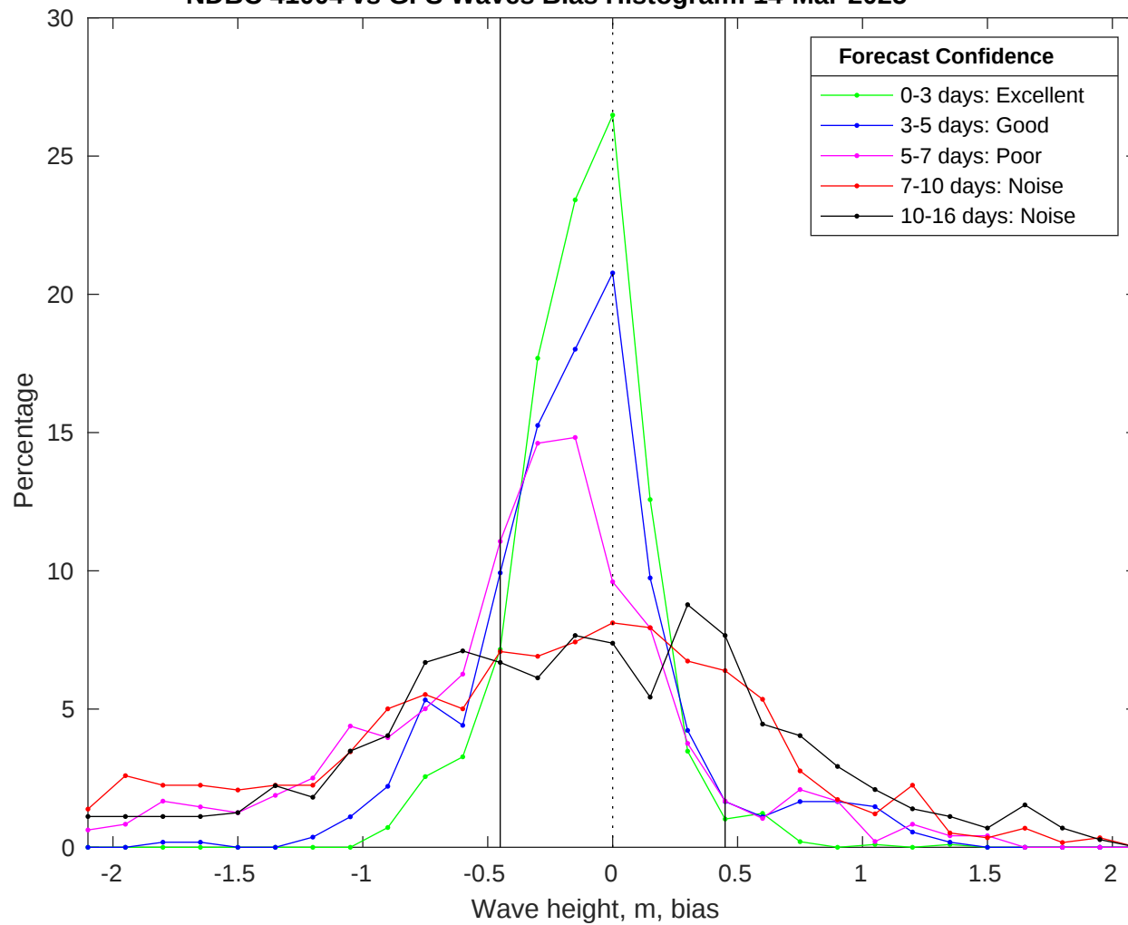
NDBC 41004 vs GFS Waves Bias Histogram: 14-Mar-2025
