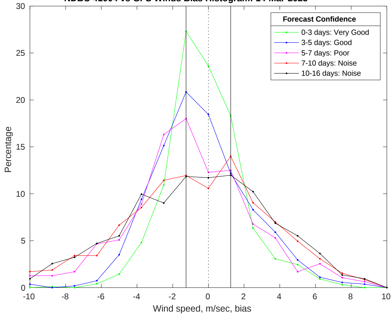
NDBC 41004 vs GFS Winds Bias Histogram: 14-Mar-2025
