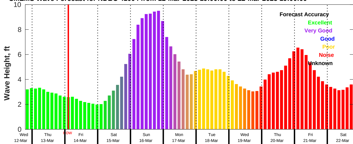
CMEMS Wave Forecast for NDBC 41004 from 12-Mar-2025 19:00:00 to 22-Mar-2025 19:00:00
